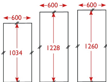
AFD60102 - H: 1034 mm AFD60122 - H: 1228 mm AFD60126 - H: 1260 mm
