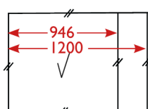
AFD9470 - B: 946 mm AFD11970 - B: 1200 mm
