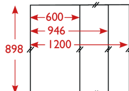
AFD6090 - B: 600 mm AFD9490 - B: 946 mm AFD12090 - B: 1200 mm
